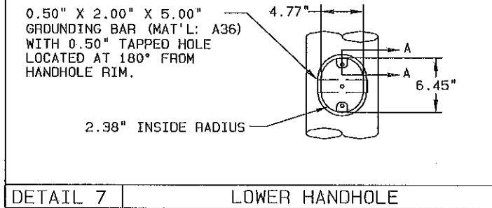
DETAIL 7 LOWER HANDHOLE
