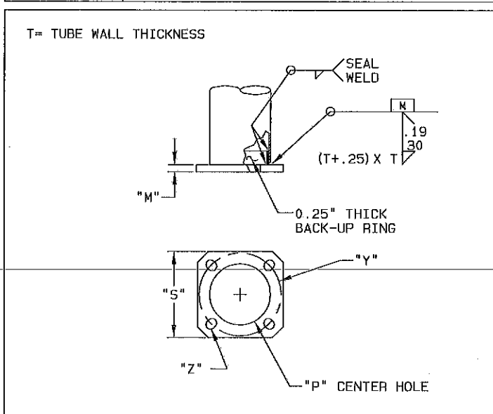
DETAIL 9 POLE BASE
