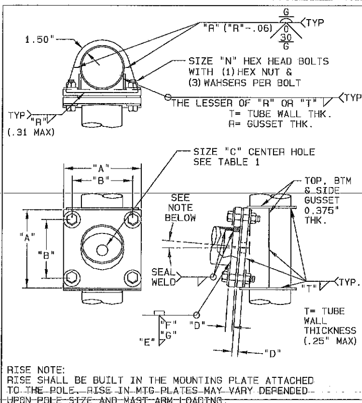
DETAIL 2 LUMINAIRE ARM ATTACHMENT
