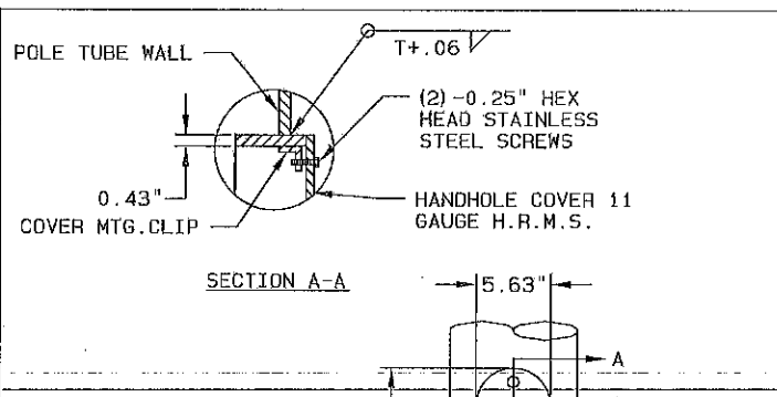
DETAIL 6 UPPER HANDHOLE
