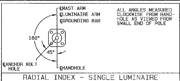
RADIAL INDEX - SINGLE LUMINAIRE
