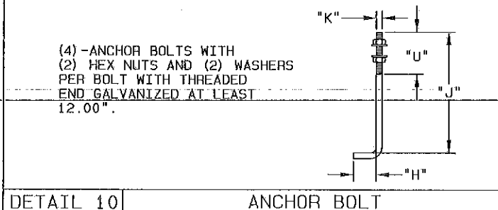
DETAIL 10 ANCHOR BOLT
