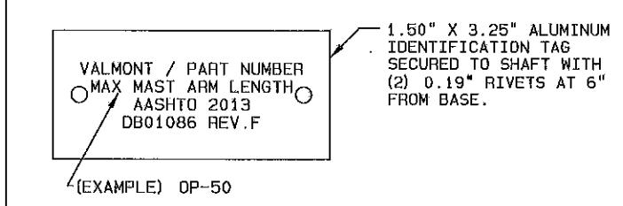
DETAIL 8 I.D. TAG
