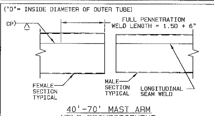
DETAIL 5 MAST ARM WELD REINFORCEMENT
