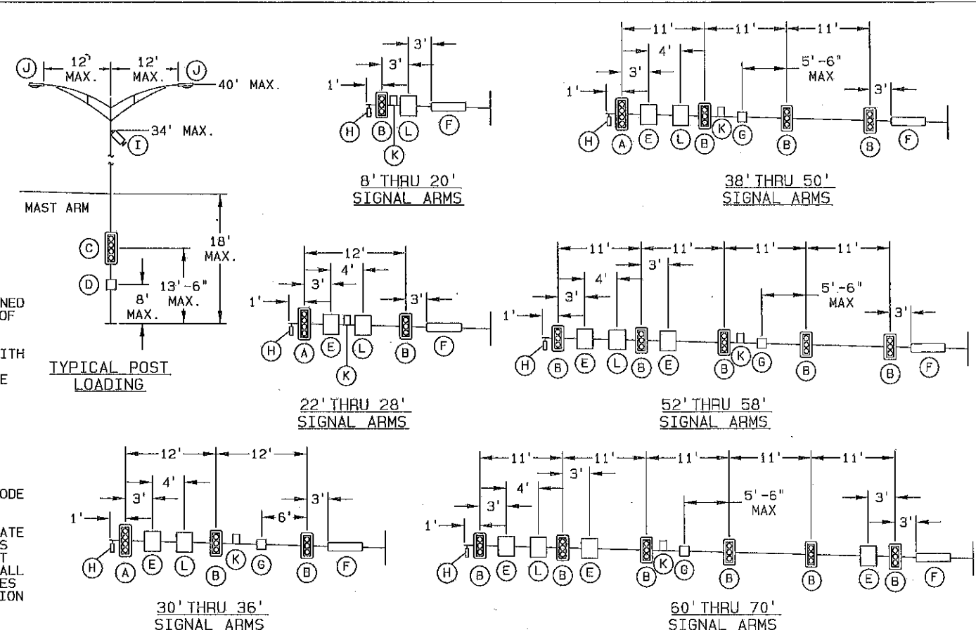
MAXIMUM LOADING INFORMATION
