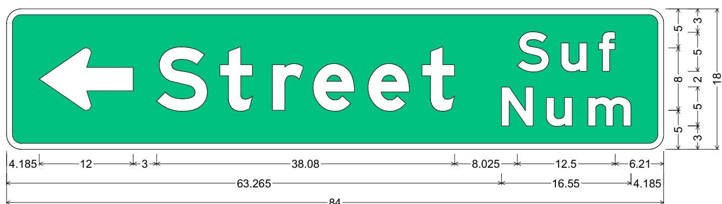
Identifier : D3-1 Sign Type : Ground Mount 1.875" Radius, 0.750" Border, White on Green; Standard Arrow Custom 0.000" X 8.000" 180"; "Street" E Mod 2K; "Suf" E Mod 2K; "Num" E Mod 2K; Table of distances between letter and object lefts.
