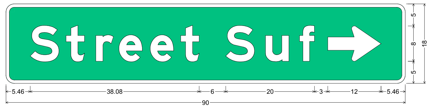
Identifier : D3-1 Sign Type : Ground Mount 1.875" Radius, 0.750" Border, White on Green; "Street" E Mod 2K; "Suf" E Mod 2K; Standard Arrow Custom 0.000" X 8.000" 0"; Table of distances between letter and object lefts.
