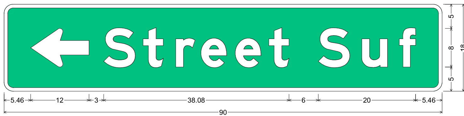
Identifier : D3-1 Sign Type : Ground Mount 1.875" Radius, 0.750" Border, White on Green; Standard Arrow Custom 0.000" X 8.000" 180"; "Street" E Mod 2K; "Suf" E Mod 2K; Table of distances between letter and object lefts.
