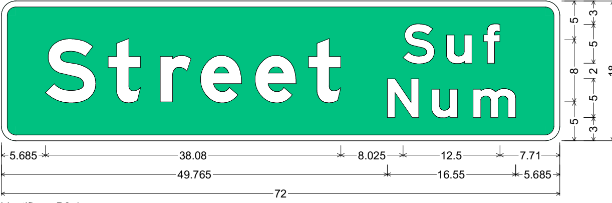
Identifier : D3-1 Sign Type : Ground Mount 1.875" Radius, 0.750" Border, White on Green; "Street" E Mod 2K; "Suf" E Mod 2K; "Num" E Mod 2K; Table of distances between letter and object lefts.
