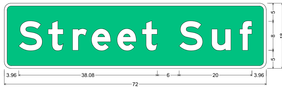
Identifier : D3-1 Sign Type : Ground Mount 1.875" Radius, 0.750" Border, White on Green; "Street" E Mod 2K; "Suf" E Mod 2K; Table of distances between letter and object lefts.
