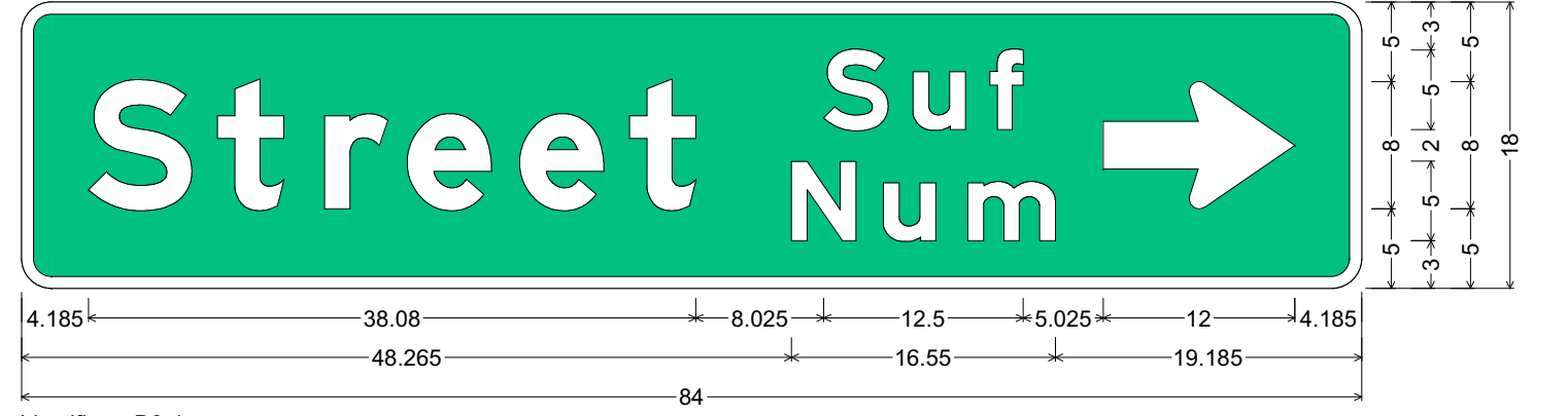
Identifier : D3-1 Sign Type : Ground Mount 1.875" Radius, 0.750" Border, White on Green; "Street" E Mod 2K; "Suf" E Mod 2K; "Num" E Mod 2K; Standard Arrow Custom 0.000" X 8.000" 0"; Table of distances between letter and object lefts.
