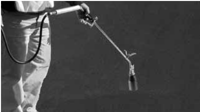
Clean the surface to remove any debris. Preheat the pavement surface to a minimum of 300° F.
