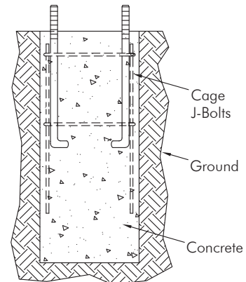
Typical Footing Detail
