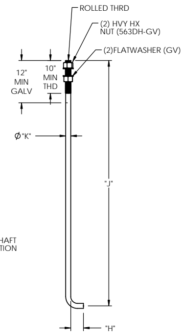
DETAIL 7 - ANCHOR BOLT DETAIL
