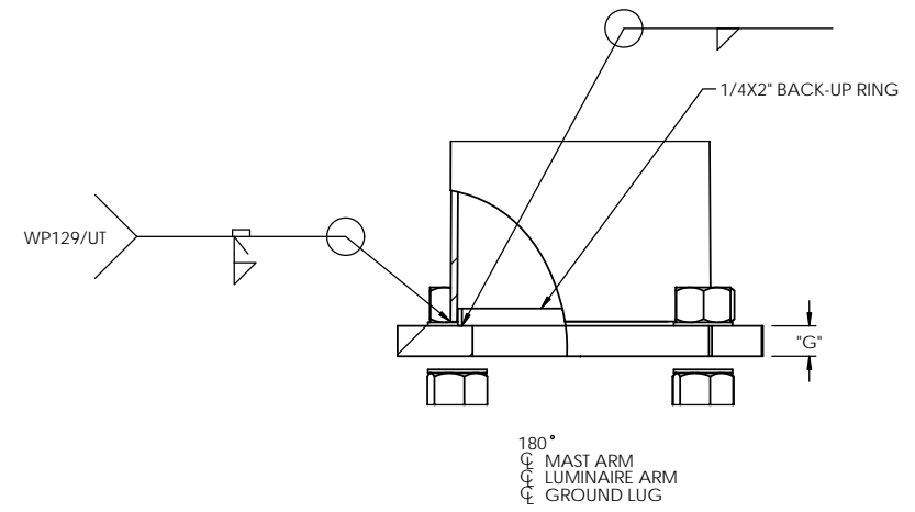
DETAIL 7 - ANCHOR BOLT DETAIL
