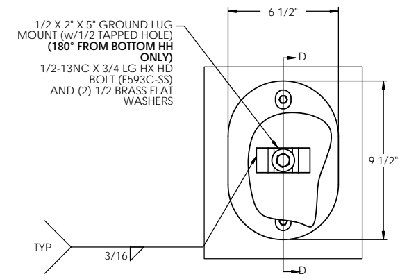
DETAIL 5 - M34 (5 X 8) HANDHOLE
