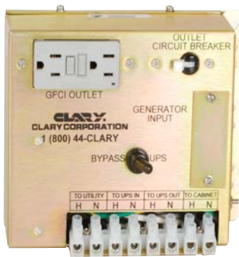
SP-PD By-pass Switch with GFCI Plug, Circuit Breaker and Generator Plug
