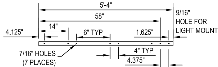
5' 4" X-TUBE
