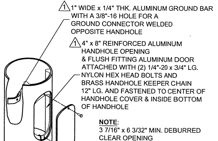
HANDHOLE DETAIL
