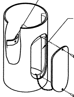
HANDHOLE DETAIL
