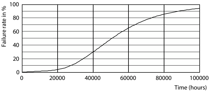
Life Expectancy Diagram - 36CC/LED/830/LS EX39 G3 BB 3/1
