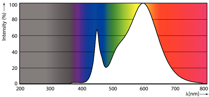
Spectral Power Distribution Colour - 36CC/LED/830/LS EX39 G3 BB 3/1
