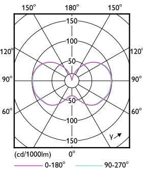
Light Distribution Diagram - 36CC/LED/830/LS EX39 G3 BB 3/1
