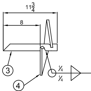
STINGER DETAIL
