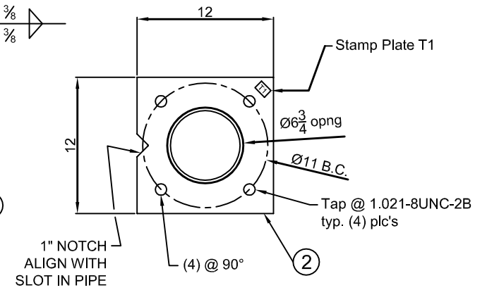
MOUNTING PLATE DETAIL
