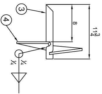
STINGER DETAIL
