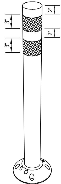
SHOWN WITH TYPICAL REFLECTIVE TAPE APPLIED
