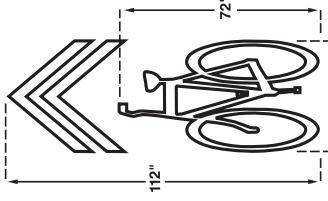
Bicycle Sharrow (SH) 112" x 40"
