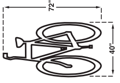
Bicycle Lane Symbol (BK) 72" x 40"
