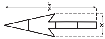
Elongated Straight Arrow (SE) 4 Pieces
