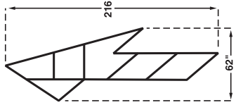
Left Lane Drop Arrow (LD) 6 Pieces
