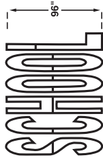
"SCHOOL" Legend (SC) 12 Pieces
