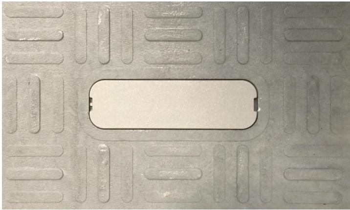
Figure 1 . Top View of Shield Lid With covered Lift Pin and 5' Ground Wire.
