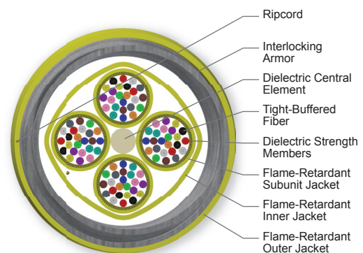
Cross Section of Part Number: 096E88-T3131-A3
