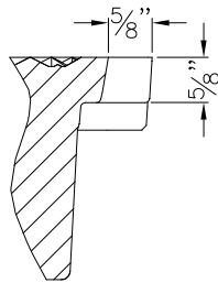
PICKHOLE DETAIL
