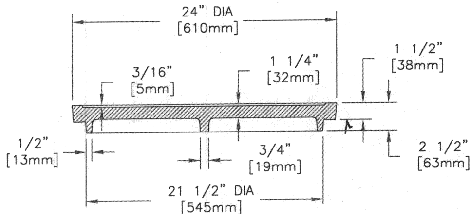
COVER SECTION
