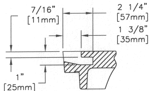
PICKHOLE DETAIL
