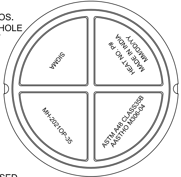
BOTTOM VIEW (COVER)
