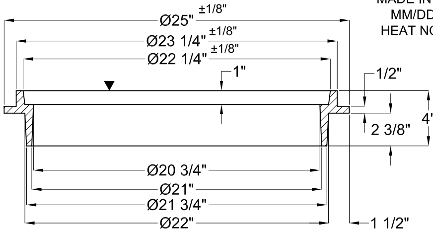
SEC. X-X (FRAME)
