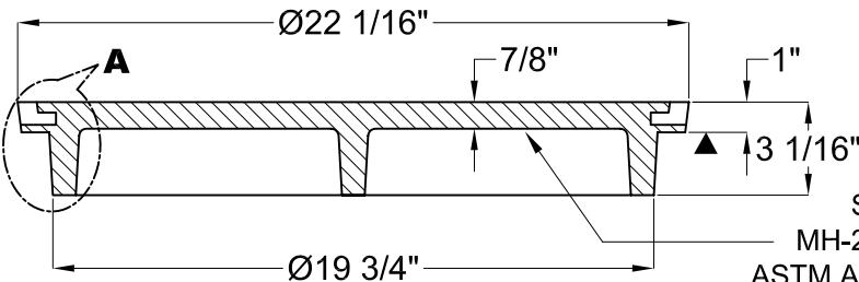
SEC. X-X (COVER)
