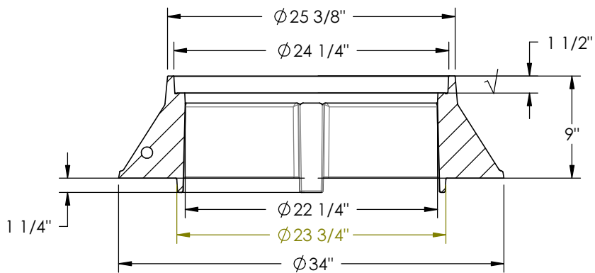
SECTION B-B
