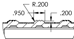
DETAIL C SCALE 1 : 4
