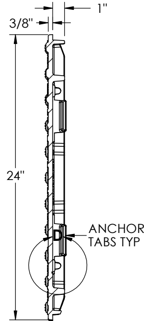
SECTION B-B
