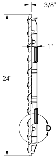
SECTION B-B
