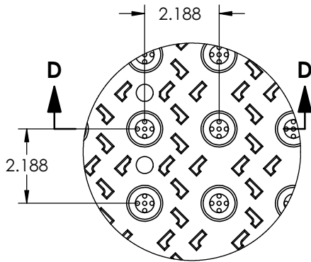
DETAIL E
