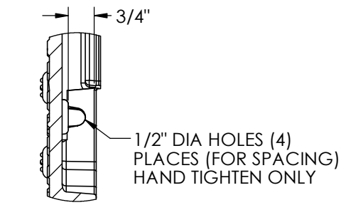
DETAIL D SCALE 1 : 4
