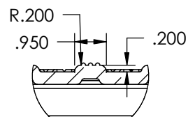
DETAIL C SCALE 1 : 4
