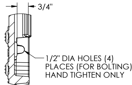
DETAIL D SCALE 1 : 4
